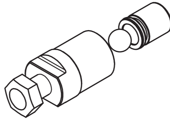
1020960211 IGNITION & STATOR TOOL
